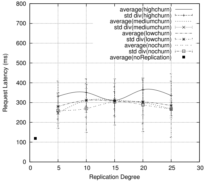
Figure 9.6: Request latency vs. replication degree
