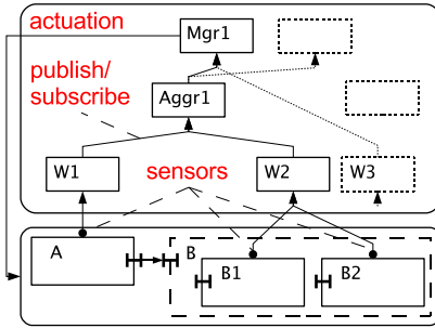
Figure 6.1: Application Architecture.
