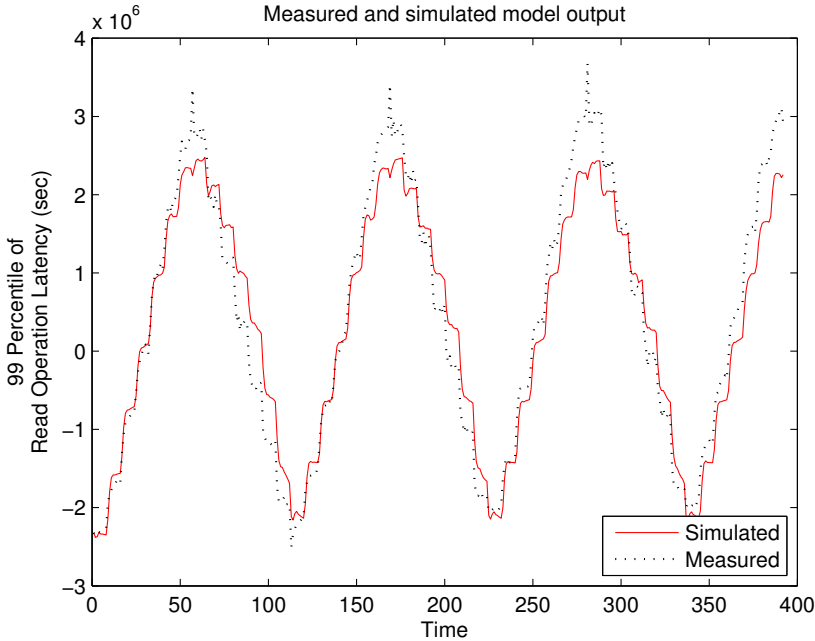
Figure 12.9: Model Performance.
