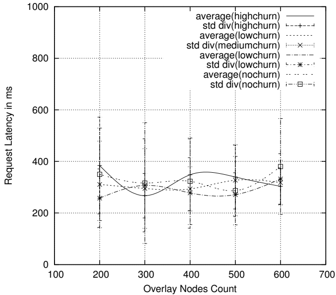
Figure 9.8: Request latency vs. overlay size
