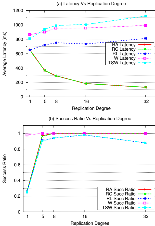
Figure 10.5: The effect of replication degree on operations
